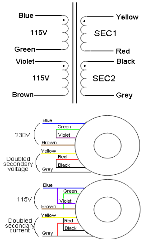
Electrical schematics
