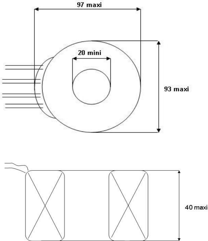
Mechanical schematics
