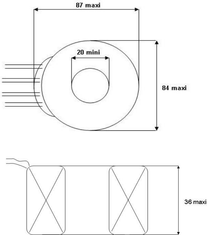
Mechanical schematics
