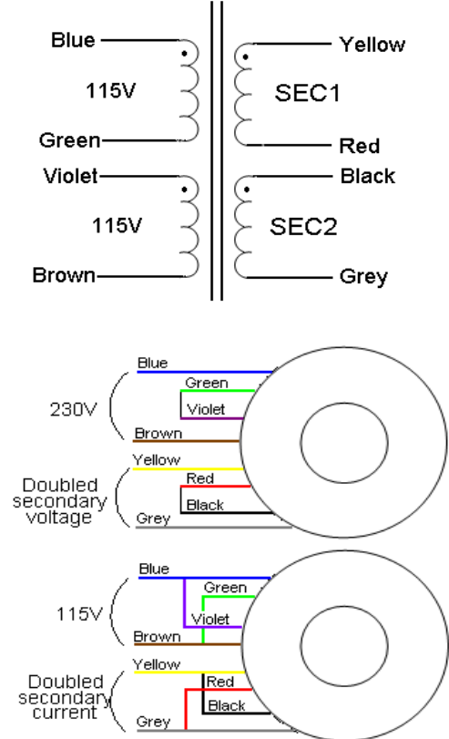
Electrical schematics
