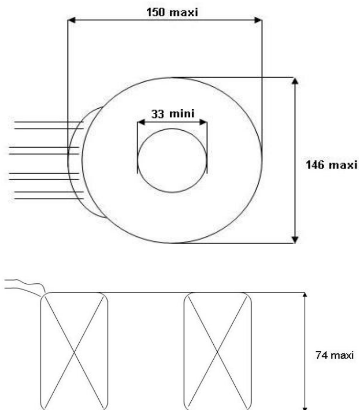
Mechanical schematics
