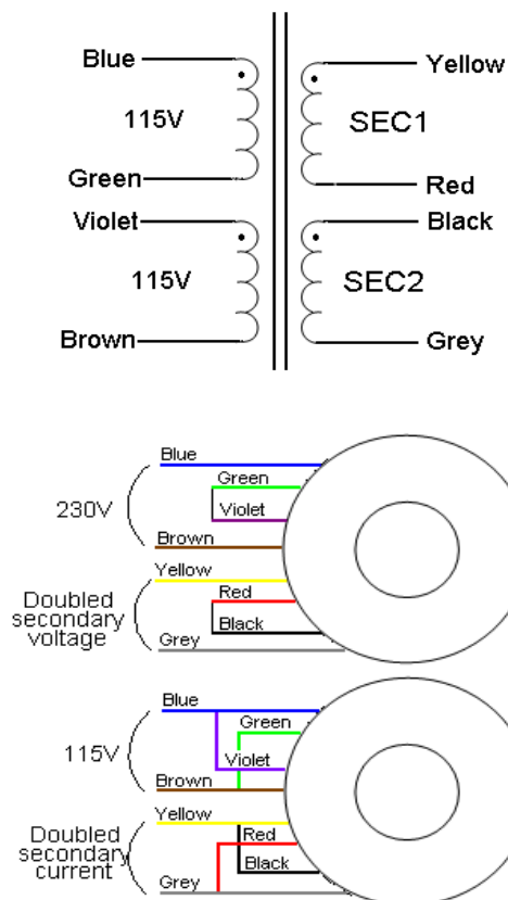
Electrical schematics
