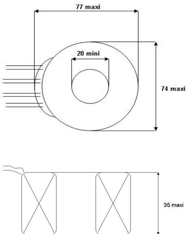
Mechanical schematics
